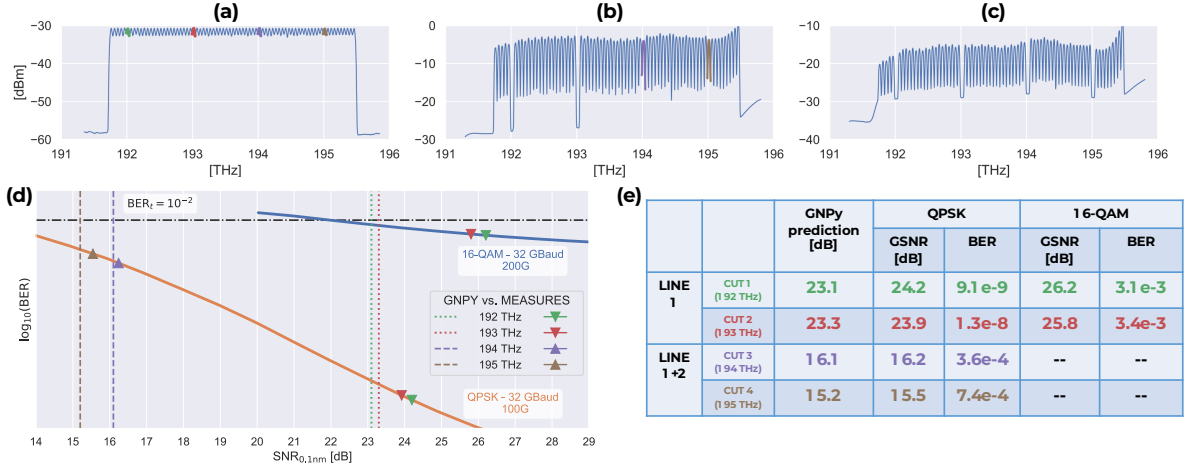
Fig. 2. Propagating WDM comb at line 1 input after ROADM 1 (a), line 2 input after ROADM 2 (b), line 2 output after ROADM 3 (c). Comparison between GNPpy predictions and experimental measurements, graphically (d) and in table (e).
