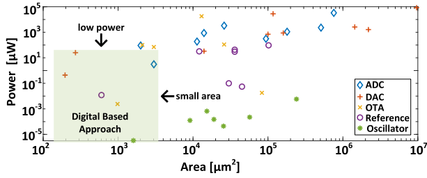
FIGURE 2. Power vs area reduction for ADCs [20], DACs [37], OTAs [54], [56], voltage reference [49] and oscillators [53], comparing traditional analog and digital-based approach.
