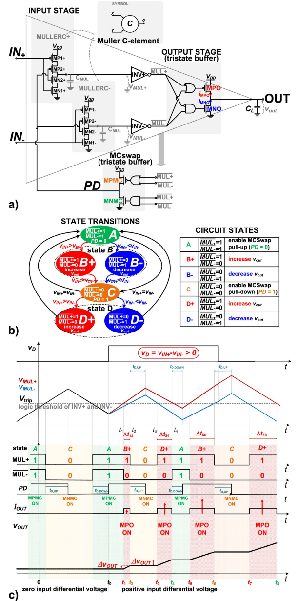
FIGURE 4. (a) Schematic of the single-end passive-less DIGOTA circuit proposed in [54]. (b) DIGOTA State-transition diagram. (c) DIGOTA circuit state and main waveforms time evolution [54].
