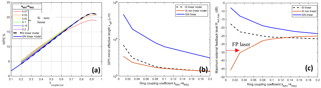
Figure2: (a) Laser WPE at P_{out}=20\text{mW} as function of the design parameters and platform (SiN or SOI); (b) SiPh mirror effective length and (c) maximum tolerated external feedback as function of the ring coupling coefficients k_{RR1,2} . In (b) and (c) T_{c,out} is fixed at 72%. The red arrow indicates the R_{ext,max} of an equivalent Fabry-Perot laser.
