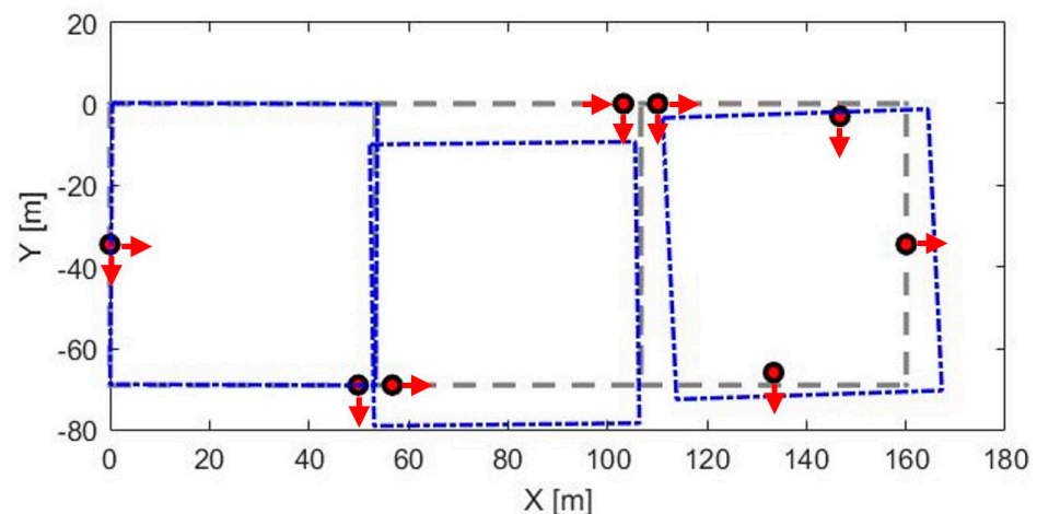
Figure 13. Identified mode shape #1 at 2.57 Hz (horizontal components).
