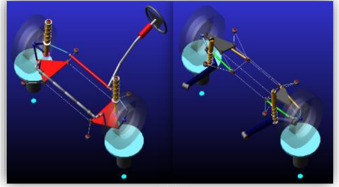
FIGURE 2 Front (MacPherson) and rear (multilink) suspension
