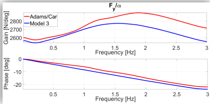
FIGURE 11 Comparison between the influence of relaxation length in Adams/Car with respect the modelled one
