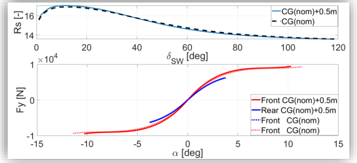
FIGURE 40 Understeer curves for different COG longitudinal positions
