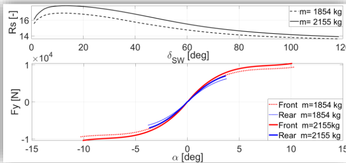
FIGURE 29 Relaxation length identification for different vehicle mass
