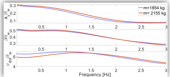
FIGURE 31 Effect of vehicle mass on the main FRFs
