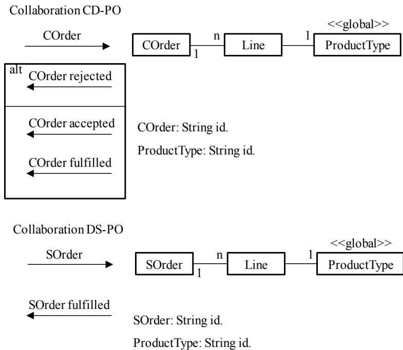
Fig.2. Collaboration models of the B2B example.
