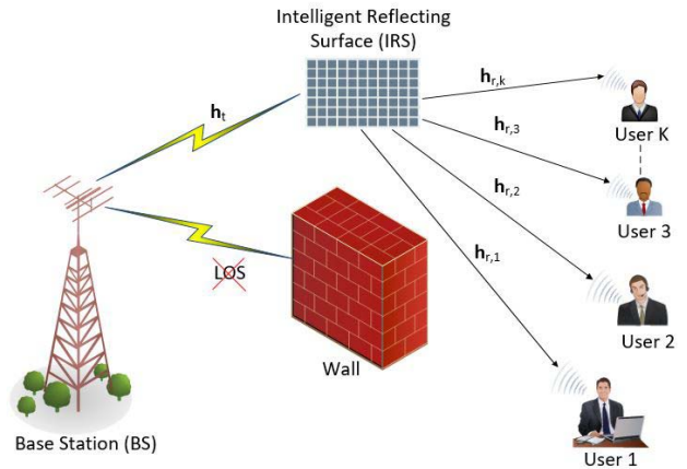
FIGURE 1. IRS assisted downlink NOMA, where the wireless communication between the BS and the endusers is accomplished through the IRS.
