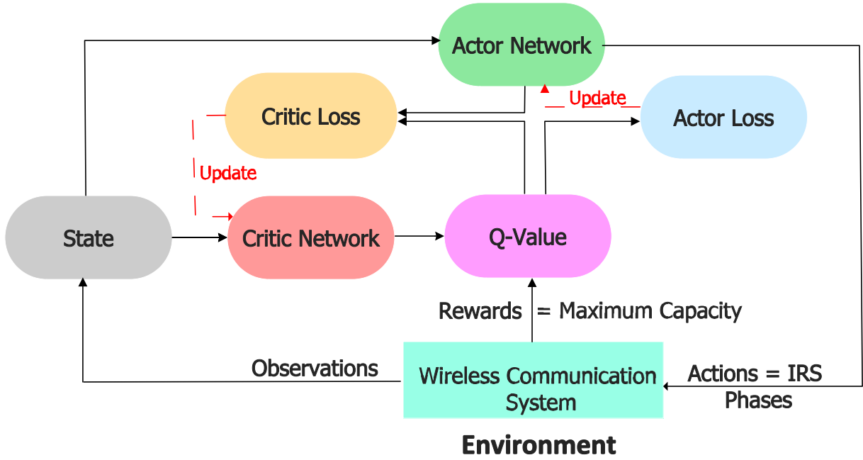
FIGURE 3. DDPG model.
