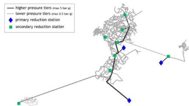
Fig. 1. Distorted representation of the topology of the distribution gas network infrastructure.
