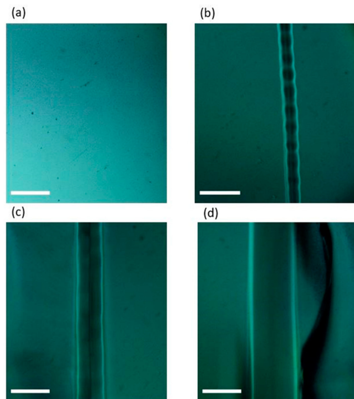
Figure 4. Micrographs of laser modification line at varying powers of 14 W (a), 16 W (b), 18 W (c), and 20 W (d), and at a fixed scan speed of 3 mm/s. Scale bar represents 50 \mu m.
