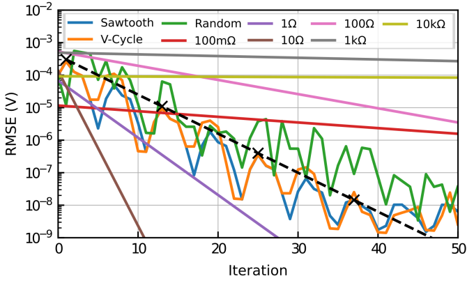
Fig. 9: As in Fig. 8, but reporting deviation \Delta v_{\text{ref}}^\nu between consecutive WR iteration steps, i.e., v_{\text{ref}}^\nu = v^{\nu-1} . The dashed black line corresponds to the proposed V-cycle IDD using v_{\text{ref}}^\nu = v^{\nu-\nu_0} .
