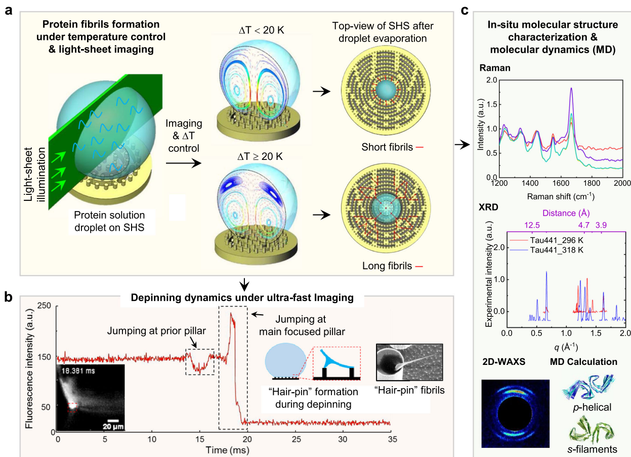
Fig. 1 Scheme of the whole process from protein fibril formation in droplet with confined convective flow field control and study of droplet contact line depinning dynamics to protein fibril molecular structure characterizations. a Protein fibrils formation with temperature gradient ( \Delta T ) controlled confined convective flow field in droplet on SHS. b Droplet contact line depinning dynamics study with ultra-fast imaging. c In situ molecular structure characterizations of protein fibrils with Raman, XRD, 2D-WAXS, and molecular dynamics (MD) calculation.
