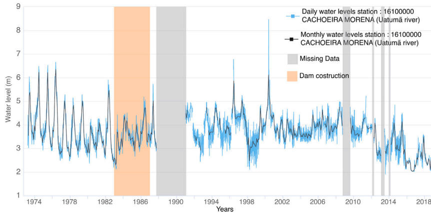
FIGURE 2 | Water levels in gauge station Cachoeira Morena.
