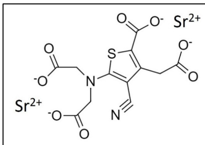
Figure 1. Strontium ranelate.
