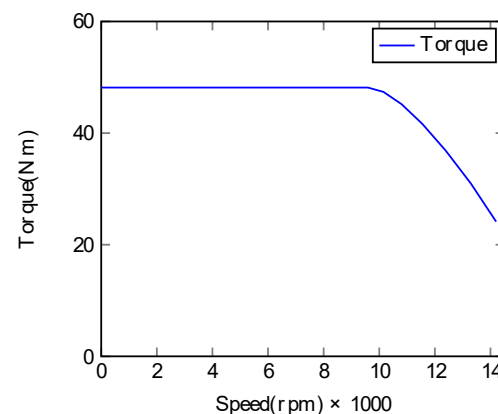
Figure 5. Torque envelope as function of the speed
