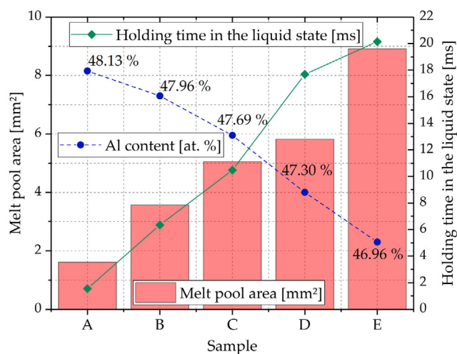
Figure 6. Calculated holding times in the liquid state (green straight line) and the melt pool area (red bars) as well as the overall Al-content (dotted blue line, see Table 1 ) drawn for the specimens A–E. With a process induced increasing holding time in the liquid state and larger melt pools, the evaporation of Al during the process does increase considerably.
