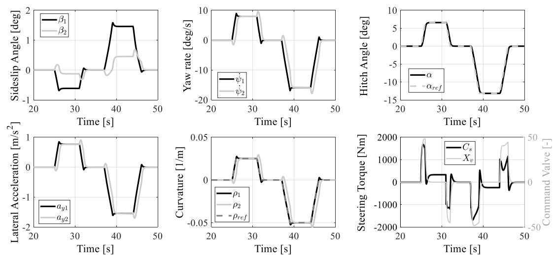
Figure 16. Sideslip angles, yaw rates, hitch angle, lateral accelerations, curvatures, steering torque, and hydraulic command valve during a multiple turn maneuver, with the hitch angle controller with SBL and fixed PID gains applied to the non-linear model at constant ATV speed u_1 = 20 km/h. Reprinted with permission from ref. [19]. Copyright 2020 Springer Nature Switzerland AG.
