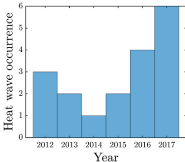
Fig. 2. Heat wave occurrence in the period 2012–2017.
