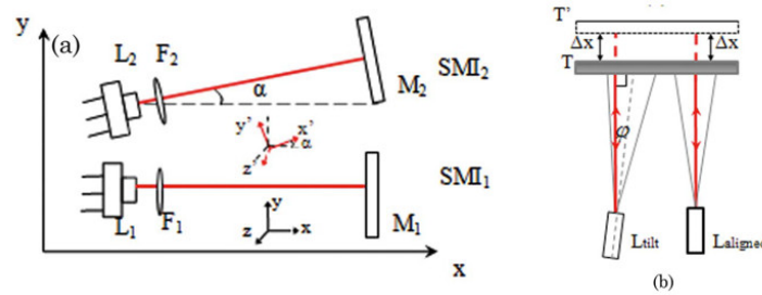
Figure 4. (a) In-plane (xy) projection of a 3D arrangement of three OF displacement sensors for simultaneous measurement of three degrees of freedom of target motion. (b) Grey lines draw the optic rays of a divergent laser beam, required to compensate the target tilt around the z-axis (adapted from Reference [32]).
