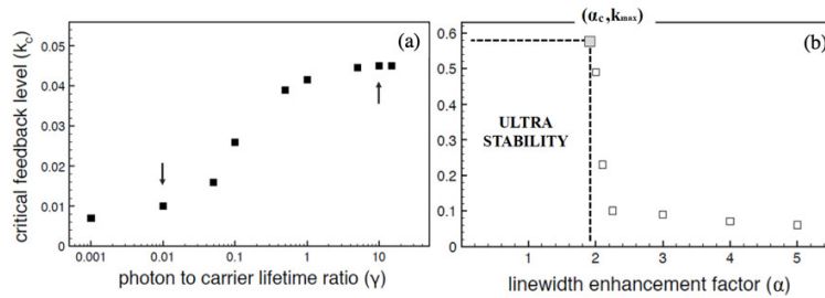
Figure 6. Dependence of the lowest feedback level \kappa_c necessary for triggering mode instability on the laser stationary emission on the lifetime ratio (a) and the linewidth enhancement factor (LEF) (b). Downward arrow in (a) marks typical value of semiconductor diode lasers, whereas upward arrow marks values of quantum-cascade lasers. (b) for \gamma = 10 , the stationary solution remains stable irrespective of the feedback level at LEF values smaller than about 2 (adapted from Reference [28]).
