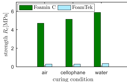
Figure 5 Effect of foaming agent on the development of the compressive strength for foamed concrete with w/c=0.3 and target dry density 600 kg/m 3 for different curing conditions
