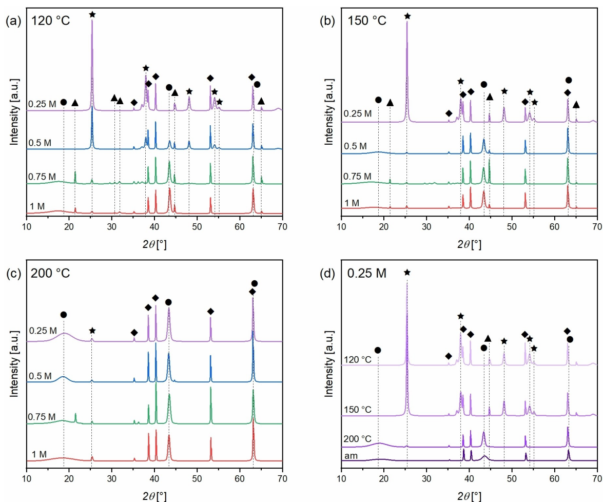
Figure 1. XRD diffractograms of the samples of TiO 2 nanotubes after the hydrothermal conversion. (a), (b), (c) Influence of temperature and concentration. Samples obtained after spending 2 hours in LiOH 0.25 M, 0.5 M, 0.75 M, 1 M at (a) 120 °C, (b) 150 °C, (c) 200 °C. (d) Effect of the temperature and phase: anatase NTs treated at 120 °C, 150 °C, 200 °C and amorphous NTs converted in LiOH 0.25 M at 200 °C. Stars (★) represent peaks of TiO 2 anatase, circles (●) the mixed oxide LiTiO x , diamonds (◆) the titanium foil and triangles (▲) Li 2 CO 3 .
