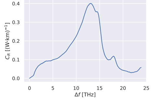
Fig. 3. Characterization results: Raman efficiency C_R(\Delta f) .
