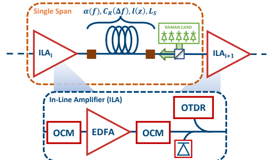
Fig. 1. Assumed optical fiber span scheme.
