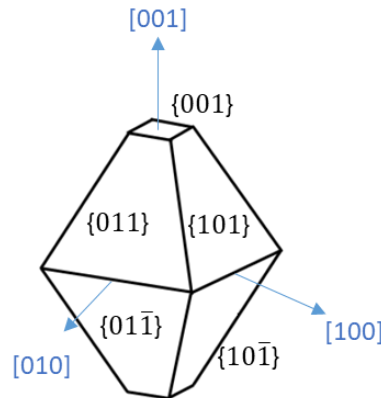
Figure 1. Equilibrium shape using Wulff construction for \text{TiO}_2 anatase crystals. Please note that in blue square brackets are reported the crystalline axes, while in curly brackets are given the anatase crystalline facets.
