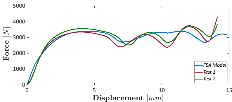
Fig. 9. Carbon Nylon lattice specimens: validation of the FEA model.
