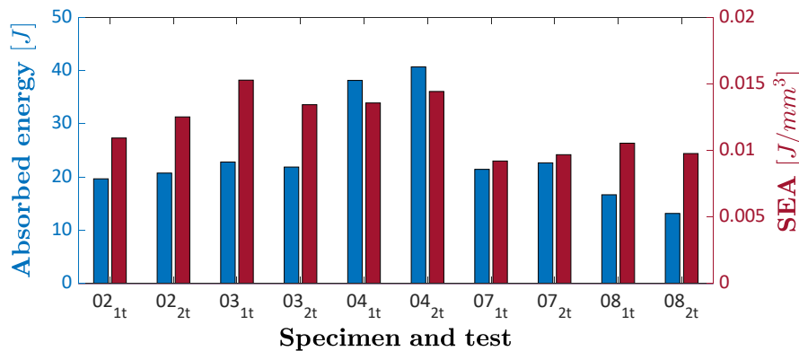
Fig. 5. Bar plot of the adsorbed energy and of the SEA for each compression test.
