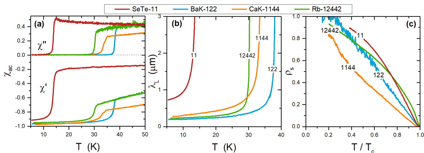
Figure 3. Comparison among different IBS families. Panel (a) shows the complex AC susceptibility of four different IBS families, 11, 122, 1144, and 12442. The penetration depth resulting from the analysis of \chi_{ac} is shown in (b). The corresponding superfluid density is shown in (c).
