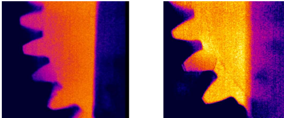
Figure 5. Thermal images of Gear 1 (left) and Gear 2 (right).
