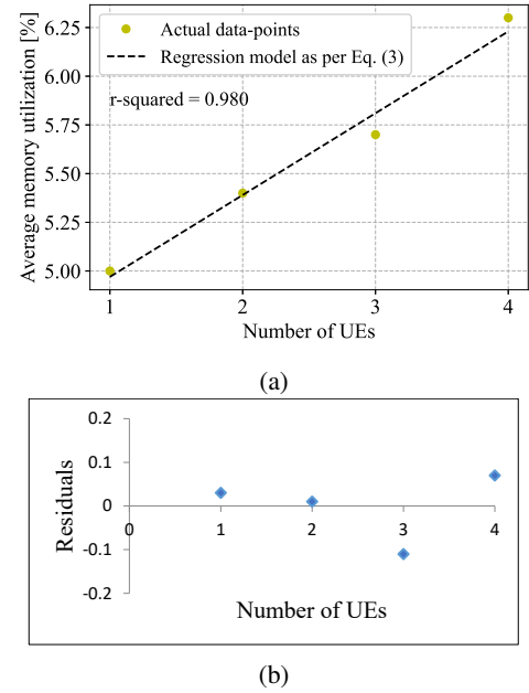
Fig. 10: Percentage of memory usage: (a) linear regression plot, (b) residual plot for MCS= 27 and 50 occupied RBs.
