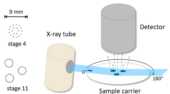
Fig. 8. On the left the patterns and dimensions of stages 4 and 11 are shown, while on the right a schematic of the TXRF spectrometer setup is reported with the arrow indicating the rotation of the sample.
