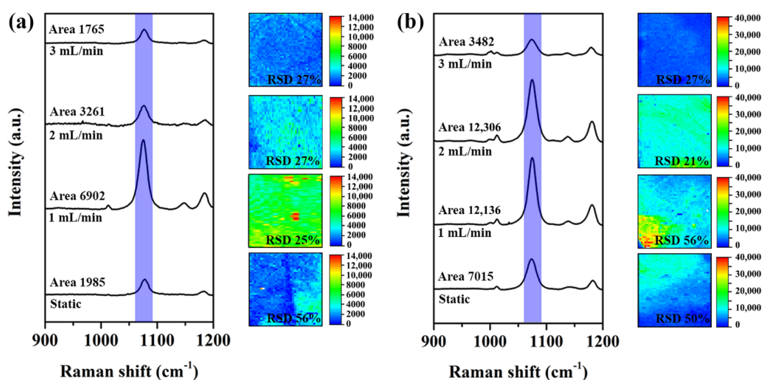
Figure 8. SERS efficiency evaluation and false colour intensity maps for the samples synthesized using (a) 10 mM \text{AgNO}_3 at 20^\circ\text{C} with different flow rates, and (b) 100 mM \text{AgNO}_3 at 20^\circ\text{C} with different flow rates. The spectra and maps corresponding to the samples prepared in static conditions are shown at the bottom of each SERS graph. The SERS spectra in this figure are the average of all the spectra collected by the mapping.
