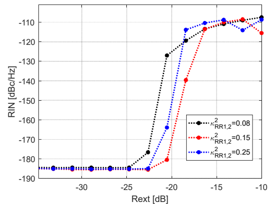
Figure 3 Integrated RIN versus external optical feedback R_{\text{ext}} at 5cm from the output port, RSOA bias to get P_{\text{out}} = 20 mW and \text{LEF} = 3 .
