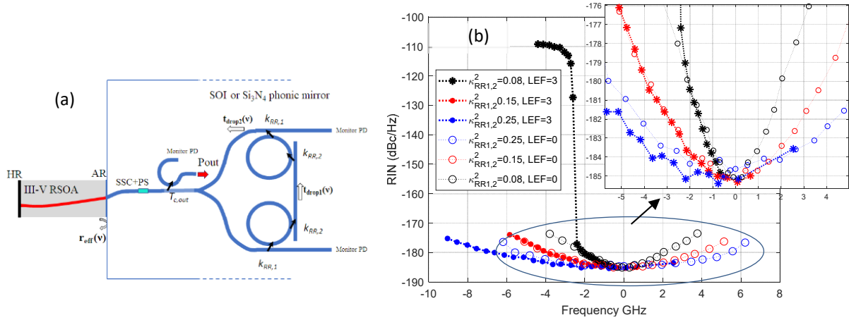
Figure 1 (a) Laser structure and (b) Integrated RIN of the output power ( \langle P_{\text{out}} \rangle = 20 mW and RSOA bias current of 104 mA) versus the detuning of lasing frequency respect to the peak of the effective reflectivity. The inset is a zoom of the region evidenced by the circle.
