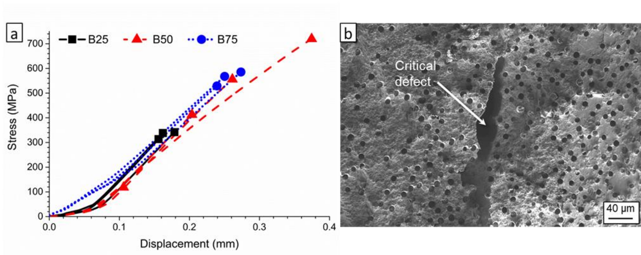
Figure 8. a) Stress/displacement curves for samples B25, B50 and B75. b) fracture surface of one of B50 bars which shows a large flaw in the material that resulted in premature failure of the specimen.
