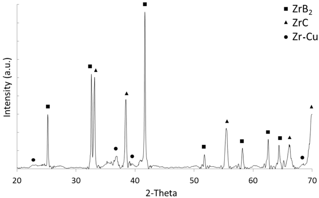
Figure 2. X-Ray diffraction pattern on the polished cross section of sample B25 after infiltration with \text{Zr}_2\text{Cu} . The phases detected were \text{ZrB}_2 (PDF#34-0423), \text{ZrC} (PDF#65-0973) and the leftover alloy \text{Zr-Cu} .
