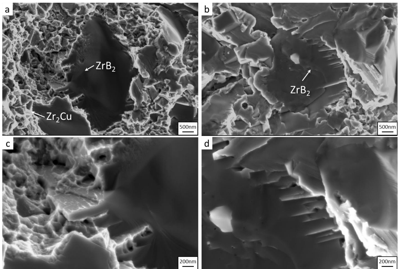
Figure 10. Fracture surface of the ceramic matrix showing the jagged \text{ZrB}_2 grains and the terraced fracture with the branches of the grains interlocking with the metallic matrix.
