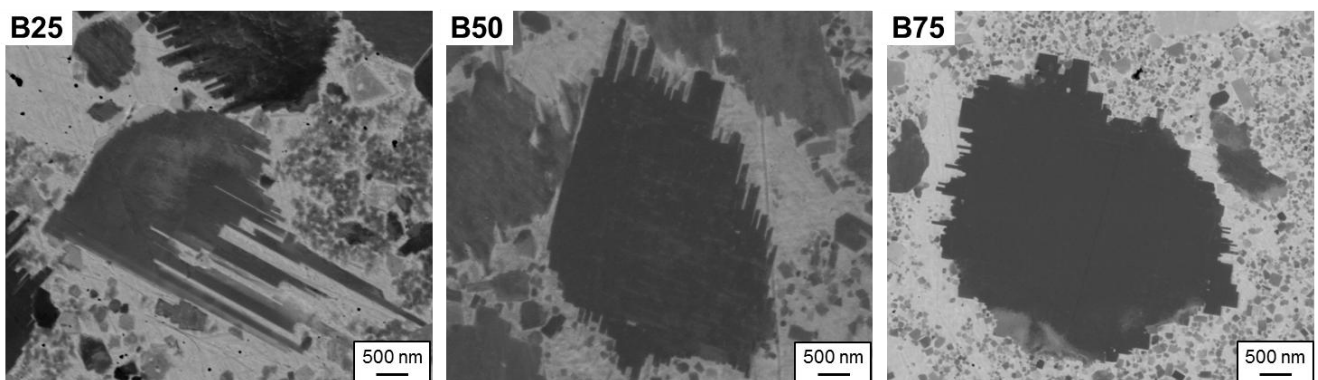
Figure 7. Detail of the jagged \text{ZrB}_2 grains. The dark and light grey phase represents \text{ZrB}_2 and \text{Zr}_2\text{Cu} respectively. \text{ZrB}_2 grain size increases with the increase of boron content.
