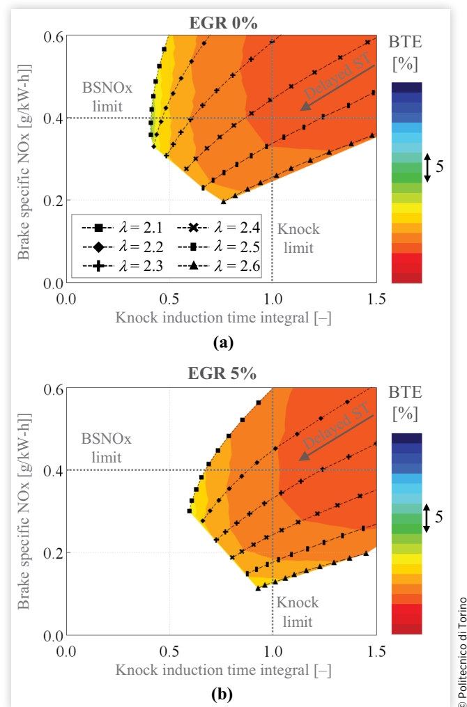
FIGURE 10 BTE obtained with different combinations of ST and lambda as a function of KITI and BSNOx for the operating point 3500 RPM \times 8 bar BMEP (a) EGR 0% and (b) EGR 5%.
