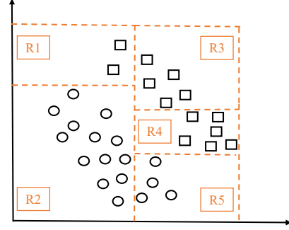
Fig. 3. An example of feature space partitioning in decision tree.
