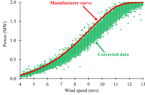
Figure 4: Corrected data vs manufacturer power curve.
