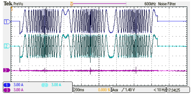
Fig. 17. Torque steps response with two active sets: phase-currents. Ch1: i_{s1,a} (3A/div), Ch2: i_{s2,a} (3A/div), Ch3: i_{s3,a} (3A/div). Time scale: 200 ms/div.
