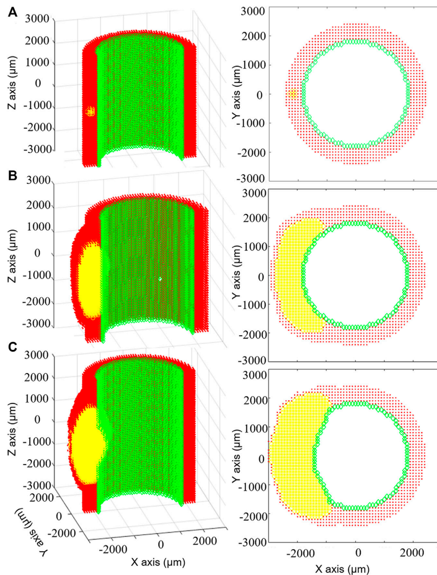
FIGURE 5 | Results of the multiscale computational fluid dynamics–agent-based model (CFD-ABM) framework of atherosclerosis by Bhui and Hayenga (2017).
