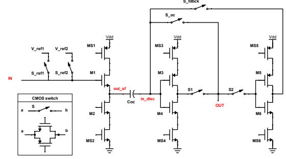
Fig. 2. Front-end circuit scheme.
