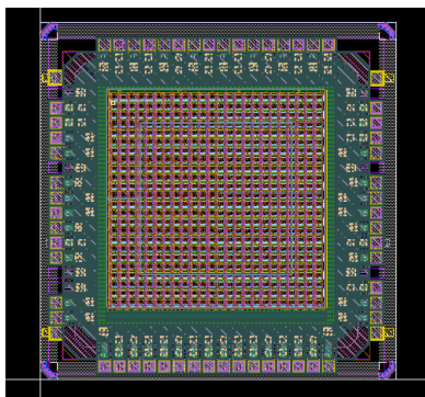
Fig. 3. First prototype, full matrix layout.
