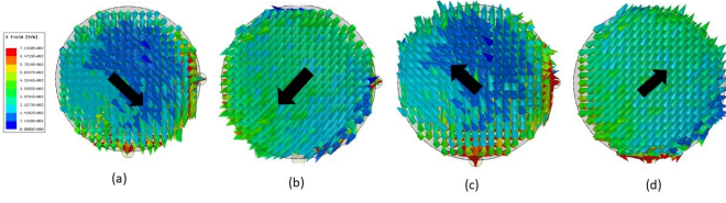
Fig. 7: Electric Field distribution in MDRA at (a) 0° (b) 90° (c) 180° (d) 270° time phase at 4.3 GHz
