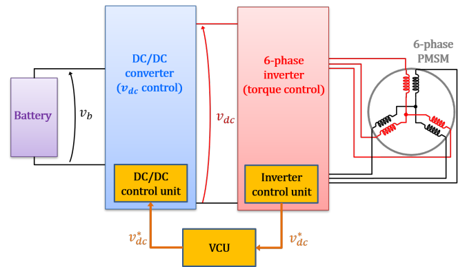
Fig. 1. Considered EV powertrain [5].
