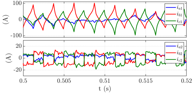
Fig. 10. Preliminary experimental results for a charging power of 5 kW.
