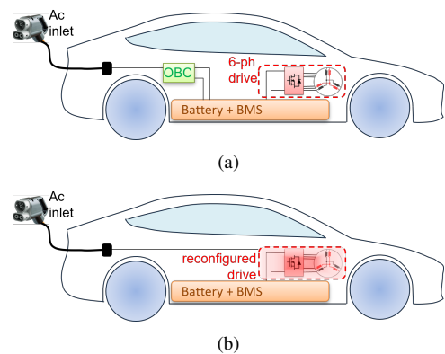
Fig. 1. On-board charger in an EV. (a) Stand-alone and (b) integrated OBC.
