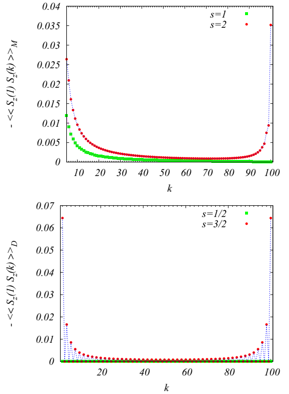
FIG. 2. Connected correlation functions, -\langle\langle S_z(1)S_z(k) \rangle\rangle , as a function of k for integer (top, for 5 \leq k \leq L ), and half-integer (bottom, for 2 \leq k \leq L ) spins for chains of length L = 100 .
