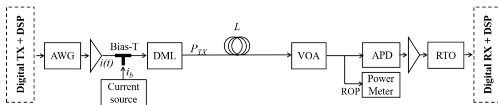
Figure 1. Experimental setup.
