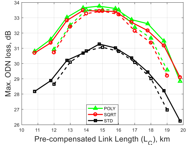
Fig. 7. Maximum ODN loss as a function of L_C with the optimum V_{pp} of driving signal. Solid: experiments with L=15.8 km and P_{TX}=11 dBm. Dashed: simulations with L=16.0 km and P_{TX}=11 dBm (dashed curves extracted from Fig.4).
