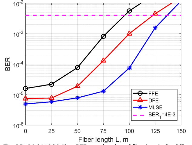
Fig. 7 PAM-4 110.35 Gbps BER as a function of fiber length, for different equalizers, using the system parameters shown in Table I. The analyzed fiber was selected from the OM3 data set in combination with VCSEL 1.
