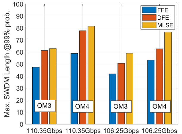
Fig. 10. Comparison of the achievable SWDM reach for 99% of the 100G links for E-FEC and KP4-FEC thresholds, and for the three equalizers.
