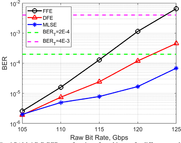
Fig. 6 PAM-4 Bit Error Rate (BER) as a function of raw bit rate, for different equalizers, using the system parameters shown in Table I.
