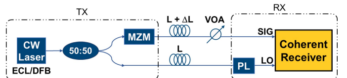
Fig. 1: Experimental setup of the self-coherent transmission system. DFB: Distributed Feedback Laser; ECL: External Cavity Laser; MZM: Mach Zhender Modulator; VOA: Variable Optical Attenuator; SIG: Signal; LO: Local Oscillator, PL: Polarization Locker.
