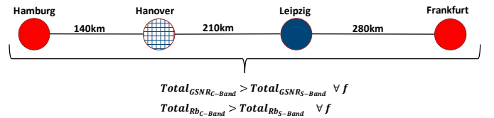
Fig. 5: Regenerator assignment description for the S-band
