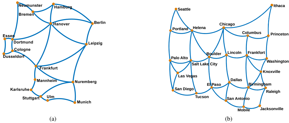
Fig. 4: (a) DT reference network's topology composed of 17 nodes with an average nodal degree of 3.1 and 26 links with an average link length of 207 km. (b) USNET reference network topology composed of 24 nodes with an average nodal degree of 3.6 and 44 links with an average link length of 308 km.
