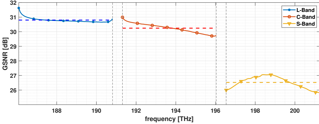
Fig. 3: GSNR profile for a single span of 70 km for L-, C-, and S-bands.
