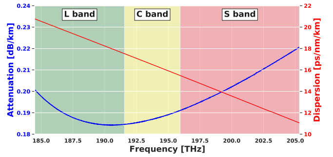
Fig. 1: Dependence of optical fiber attenuation and dispersion coefficients on frequency for a typical standard single-mode fiber (SSMF).
