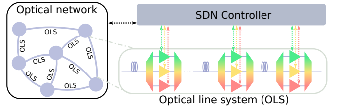
Fig. 2: Illustration of a multi-band OLS amplification.
