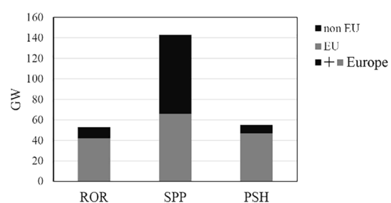
Fig. 2. (a) Annual energy generation (a) and installed power (b) in EU and Europe.
