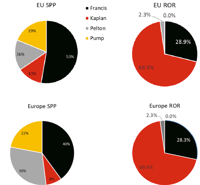
Fig. 3. Estimated turbine prevalence in EU and Europe.
