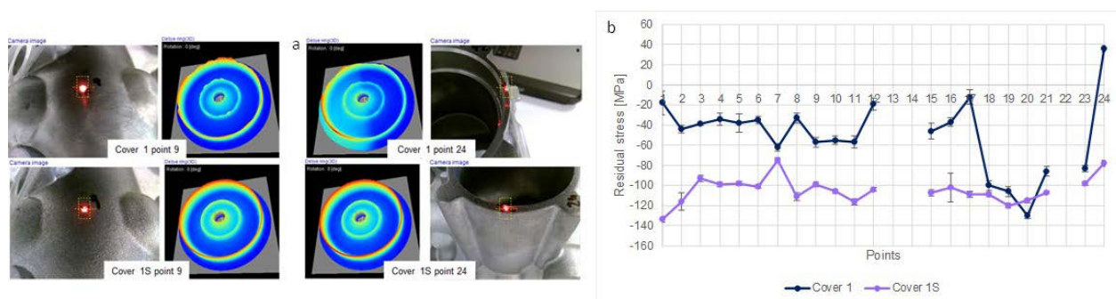
Fig.3 - a. Results obtained for 'thin large valve cover' in the as-cast state (Cover 1) and after shot blasting (Cover 1S). Upper images: points #9 and #24: Debye rings and camera images of the referred points. b. line chart of measurements performed.
