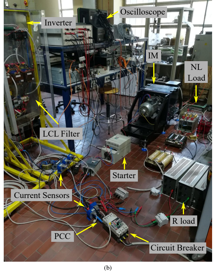
Fig. 4. Pictures of the experimental setup.
