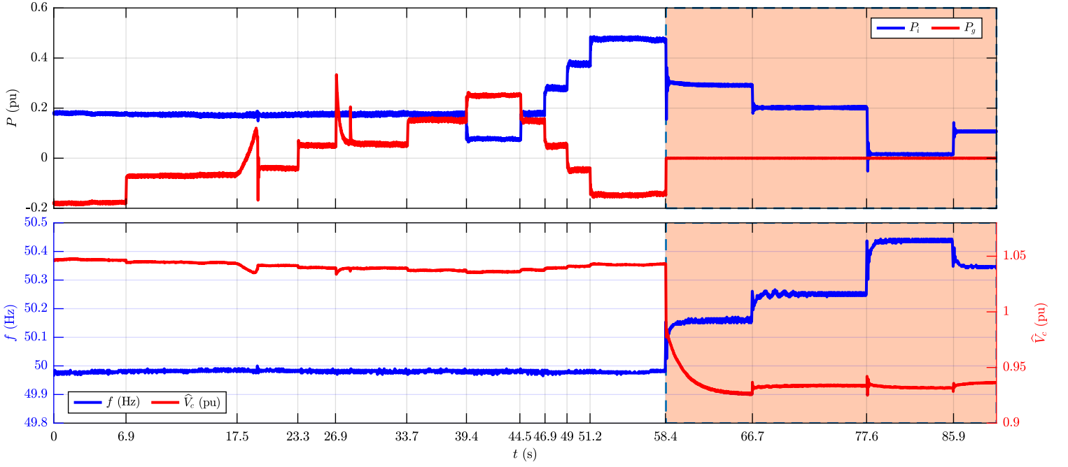
Fig. 7. Results of Test 2: (top) inverter power P_i (pu) and grid power P_g (pu) moving average trends; (bottom) S-VSC frequency f (Hz) and voltage amplitude \hat{V}_c (pu) trends.
