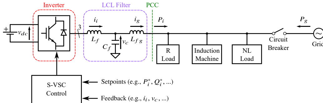
Fig. 1. Block scheme of the microgrid under study.
