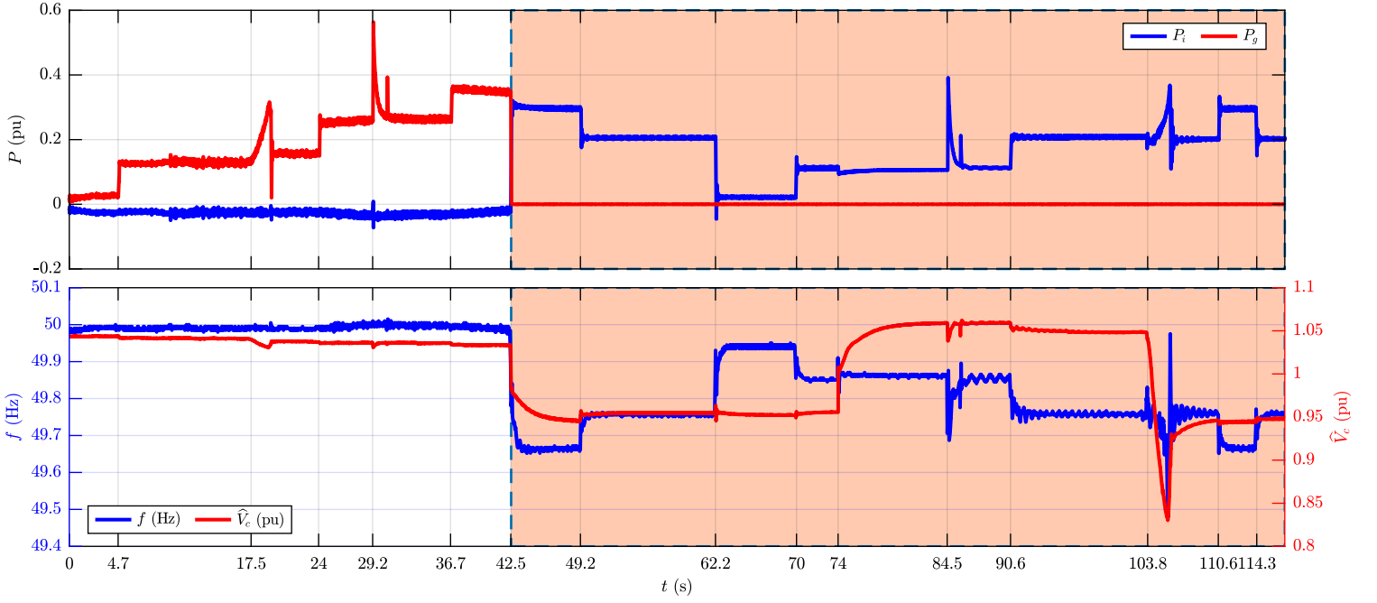
Fig. 5. Results of Test 1: (top) inverter power P_i (pu) and grid power P_g (pu) moving average trends; (bottom) S-VSC frequency f (Hz) and voltage amplitude \hat{V}_c (pu) trends.
