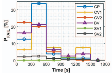
Fig. 3 Conditional probability of failure P_{FAIL,l}(e|c) (9) of each component e for cluster c=4 , as a function of time l
