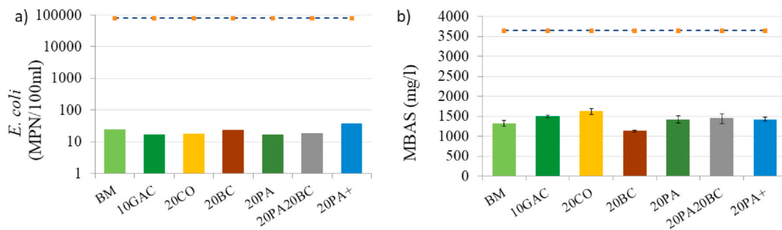
Fig. 5. Average values of concentration of a) E. coli and b) MBAS of input GW (dashed lines) and outlet of all filter media mixes. Filter medium mixtures are denoted as (see text for further details) BM: base medium; 10GAC: granular activated carbon; 20CO: compost; 20BC: biochar; 20 PA: polyacrylate; 20PA20BC: polyacrylate and biochar; 20 PA+: polyacrylate (old configuration).
